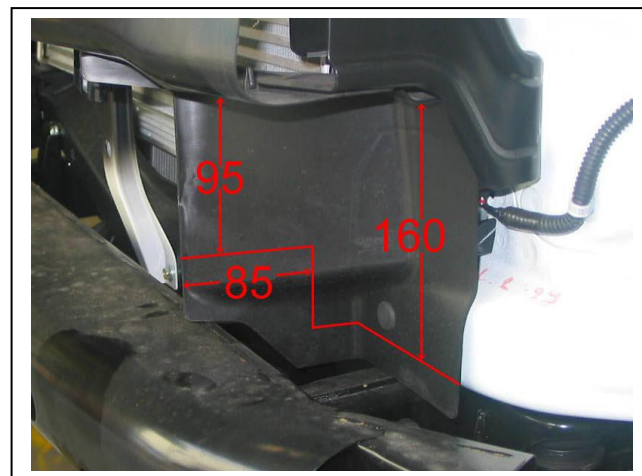
Figure 4: Measurement for air dam trim.
